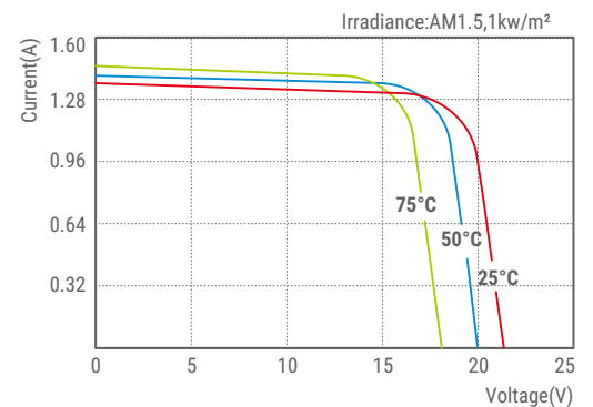
SLP020S-12U I-V Curves
